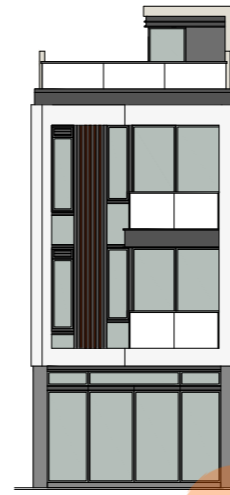
立面圖 B (適用於 B1, B3, B6, B9, B11, A3, A6, A8, A10 和 A11洋房) Elevation Plan B (For Houses B1, B3, B6, B9, B11, A3, A6, A8, A10 & A11)
