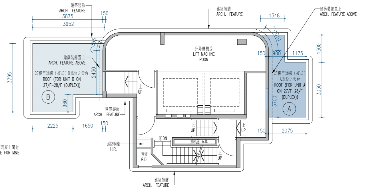
Lower Roof Plan 下層天台平面圖
