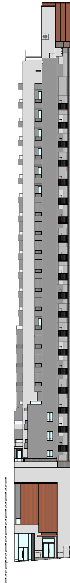
SOUTH-WEST ELEVATION PLAN C 西南面立面圖 C
