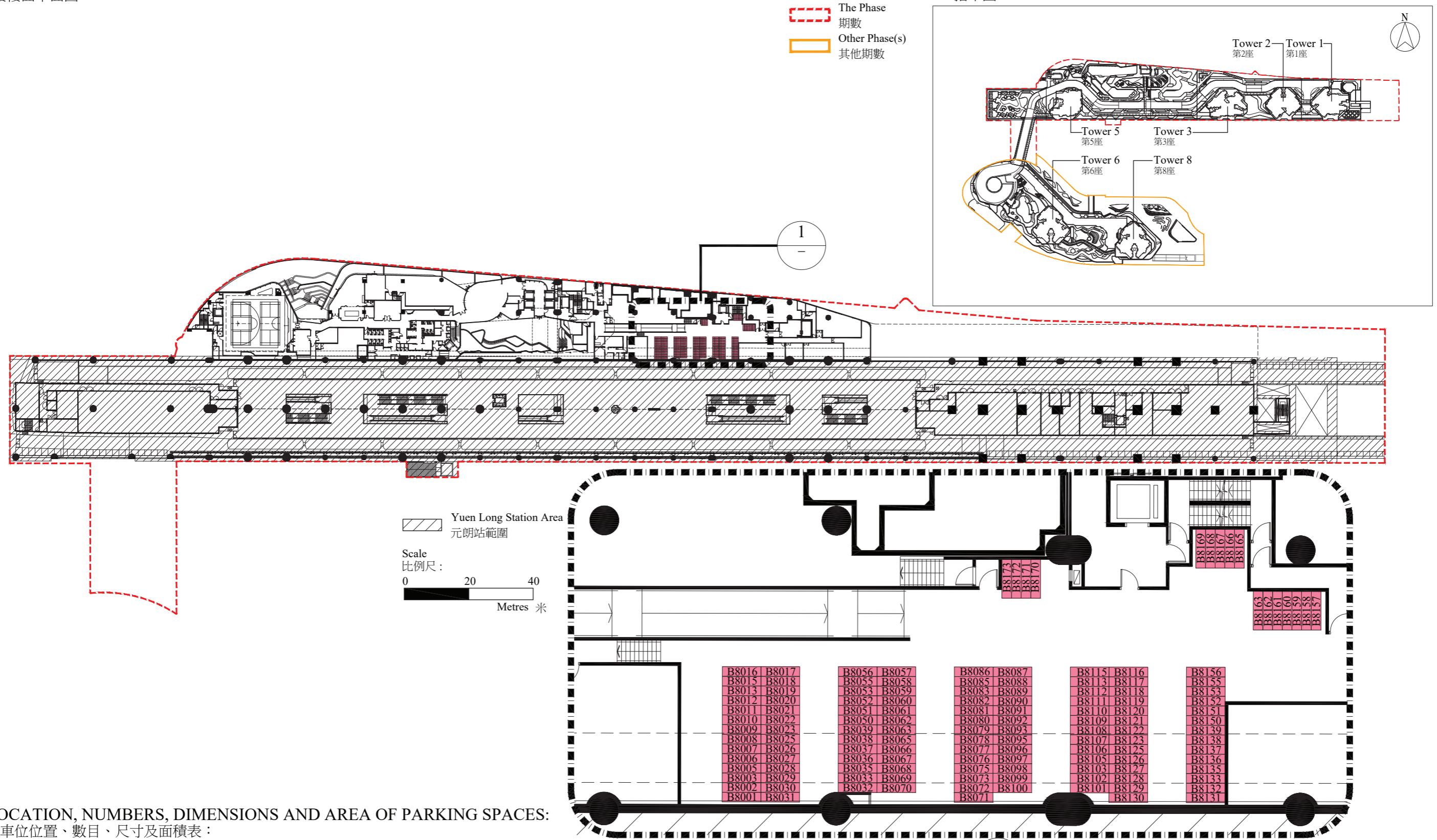
1 Part Plan of Residential Bicycle Parking Spaces 住宅單車停車位局部平面圖
