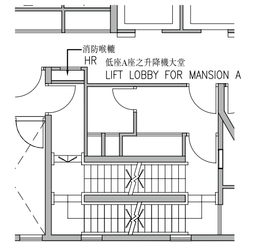
Part Plan of Lift Lobby for Mansion A on 5/F 5樓低座A座之升降機大堂之部份平面圖
